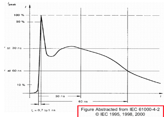
Figure 14. IEC 61000-4-2 Electrostatic Discharge
